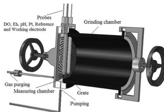
Fig. 1. Schematic representation of specially designed ball mill
