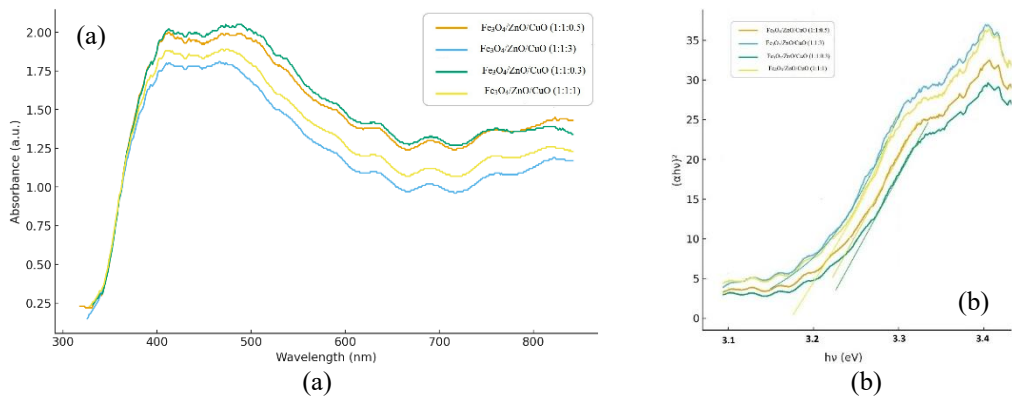
Fig. 6. Bandgap analysis curves of Fe 3 O 4 /ZnO/CuO nanocomposite: a) UV-VIS Absorption Spectra, b) Tauc's plots graphs ( n= 2 )
