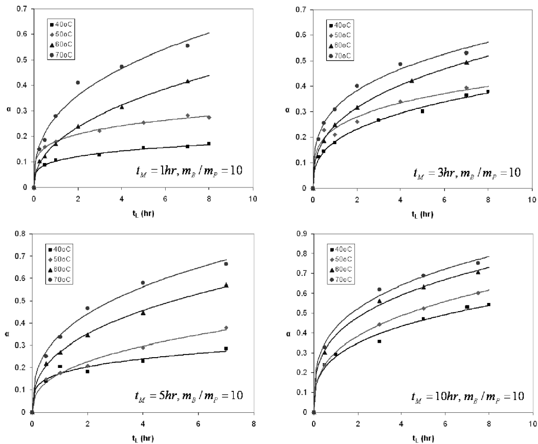
Fig. 1. Typical leaching curves of the activated chalcopryrite.
