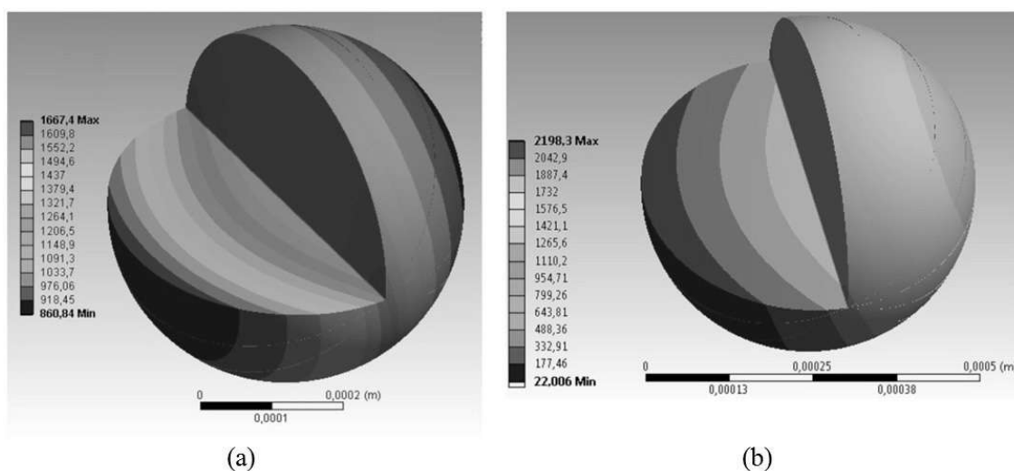
Fig. 5. Particle temperature distribution: (a) V = 5 \text{m/s} , P = 2200 \text{W} , (b) V = 4 \text{m/s} , P = 1500 \text{W}
