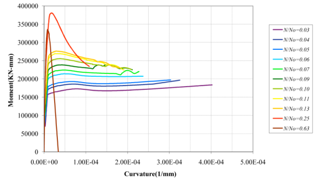
Fig. 6. Influence of axial load on descent of ultimate curvature
