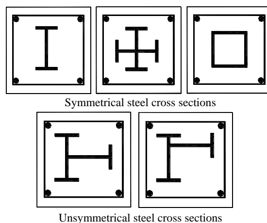
Fig. 1 Types of concrete-encased steel composite column
