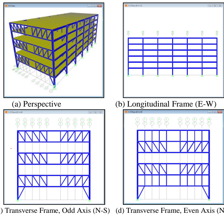
Fig. 4 Building Modeling With STF System
