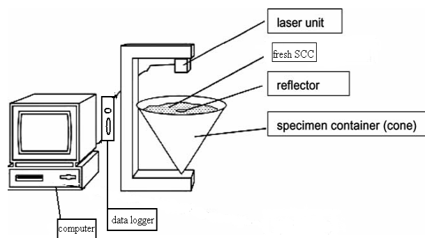
Fig. 3. Picture of test apparatus and the setup for measurement of early age shrinkage
