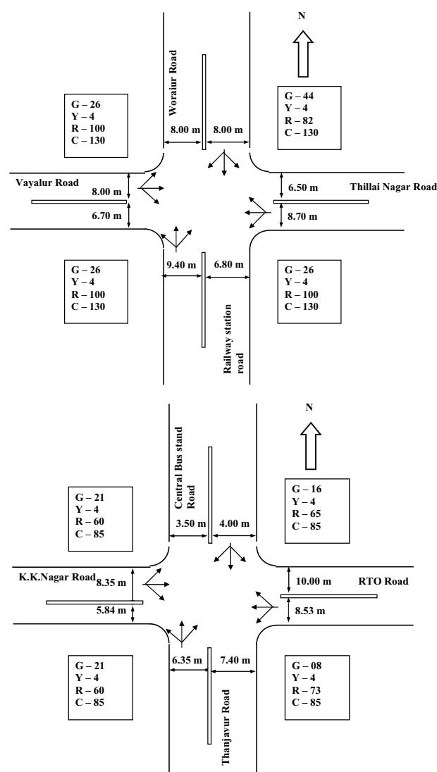
Fig. 2 Layouts of study intersection 4 and 5
