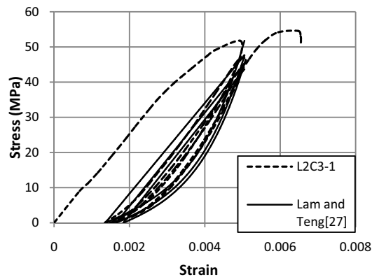
Fig. 13. Comparison between Lam and Teng model and test results
