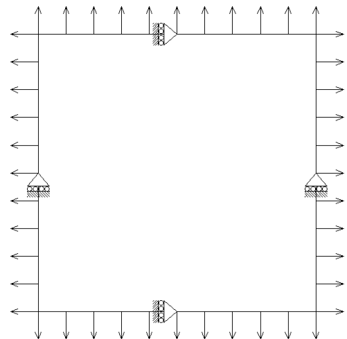
Fig. 10. Virtual constraints required for Finite Element solution
