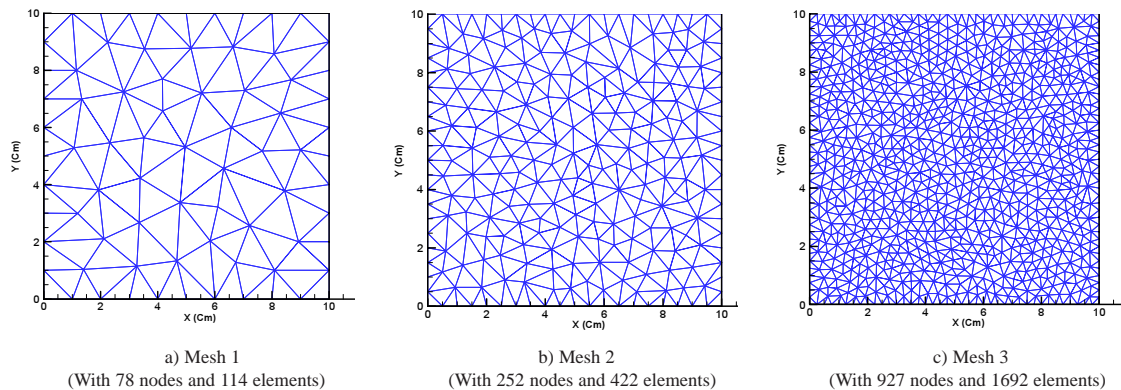
Fig. 13. Different mesh refinements for stress analysis
