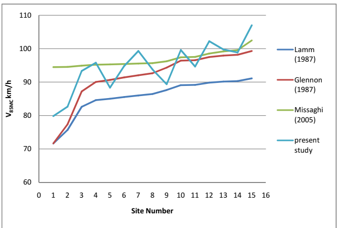
Fig. 6. Comparison of the predicted values of V_{85MC} from model developed in this study and with those from previous research
