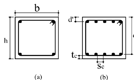
Fig. 2. Limitations of the reinforcement of the column sections (a) At least 4 longitudinal bars at four corners of the section (b) Symmetric pattern of the bars and the distance and cover of the reinforcing bars
