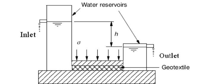
Fig. 1. Schematic side view of the transmissivity test equipment
