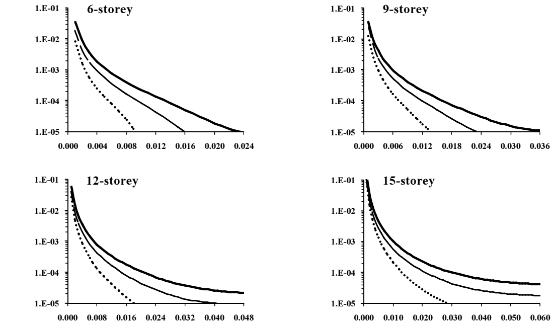
Fig.6. Determined drift hazard curves of SMRFs for territory of Tehran city in three different seismic zones, using one-parameter PSDM No02
