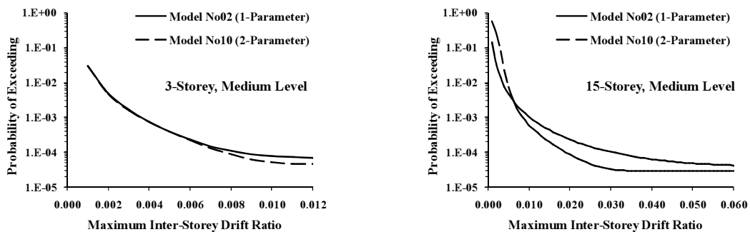
Fig. 7. Comparison of estimated seismic drift demand in 3 and 15-storey frames through using one-parameter model No02 and two-parameter model No10
