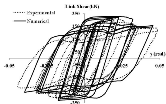
Fig. 5. Comparison of experimental and analytical link shear versus link rotation
