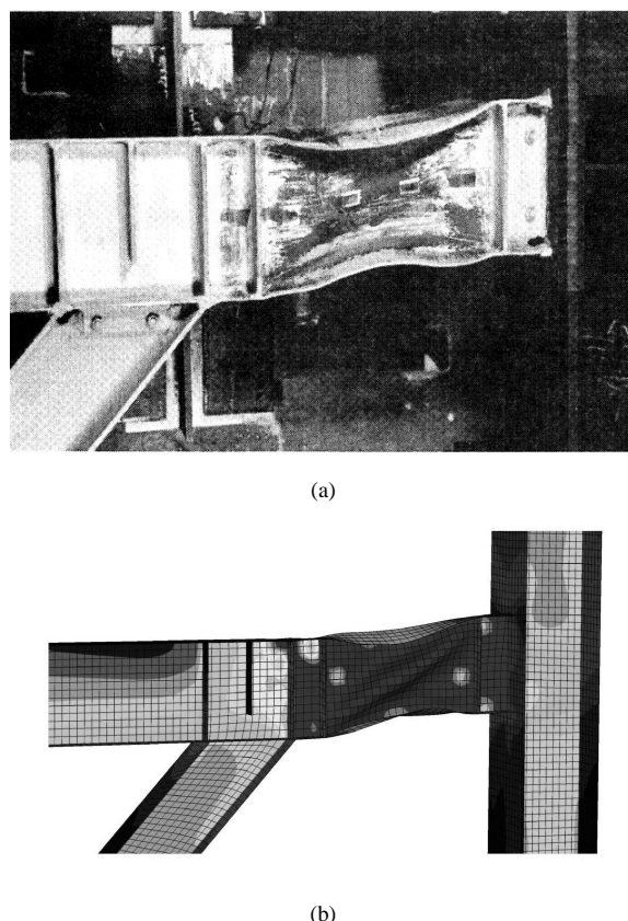
Fig. 6. Specimen after testing (a) Engelhardt and Popov (1989) (b) finite element analysis results
