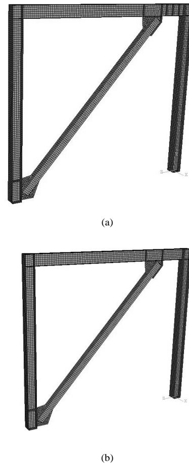
Fig. 8. Finite element model of one of designed eccentrically braced frame with (a) Carbon Steel (b) Easy-Going Steel
