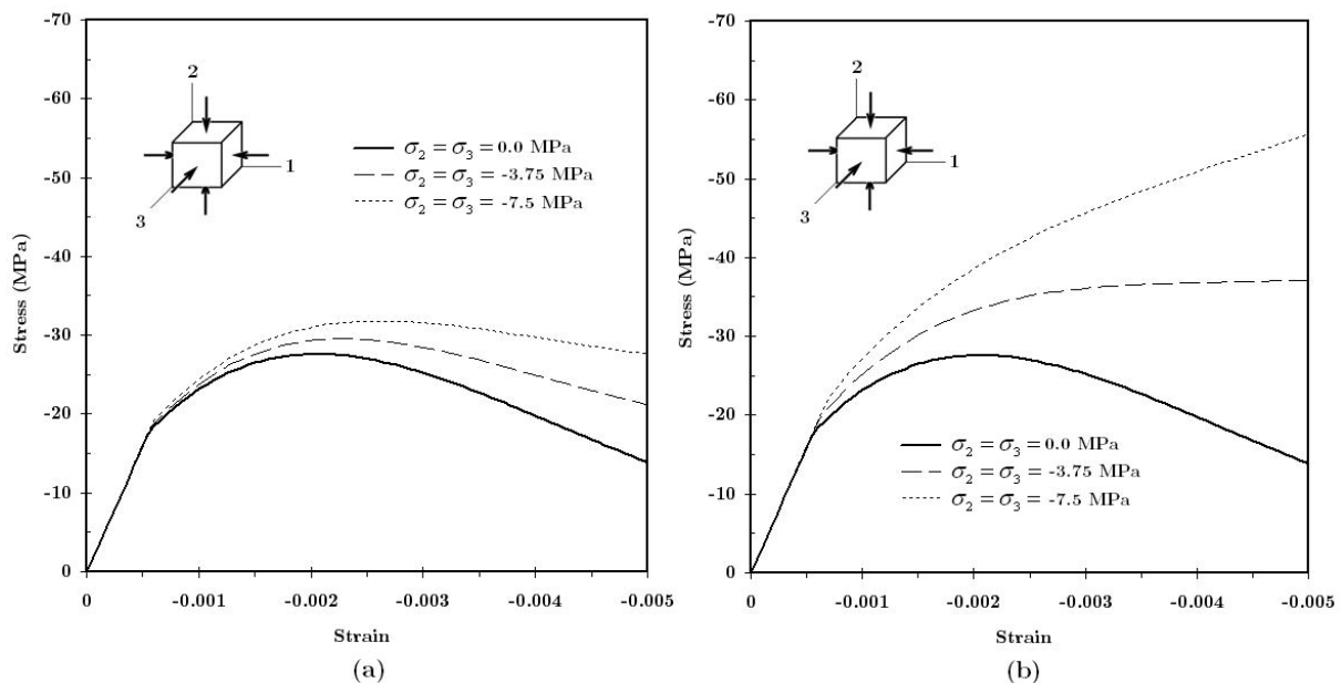
Fig. 6. \sigma_1 - \varepsilon_1 curves under three different confinements: (a) \gamma = 0 and (b) \gamma = 3
