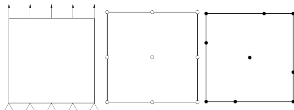
Figure 1 The patch test: a rectangle under uniform tension. The two nodal configurations
